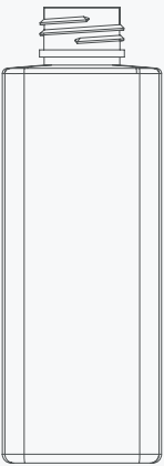
SB180 H128.9 x W(45x45)mm 24/410-25g 200ml PET
