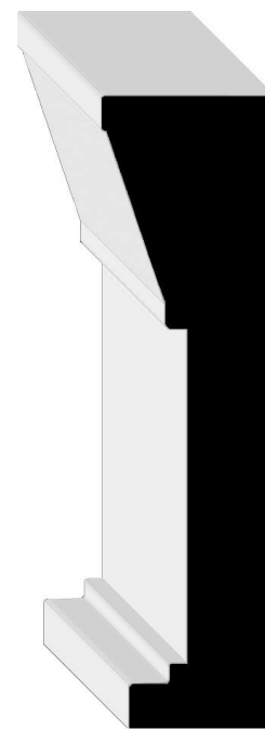
1 1/2" x 5 1/2" MODERN ARCHITRAVE
