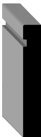
3 1/2" x 5/8" CRAFTSMAN CASING
