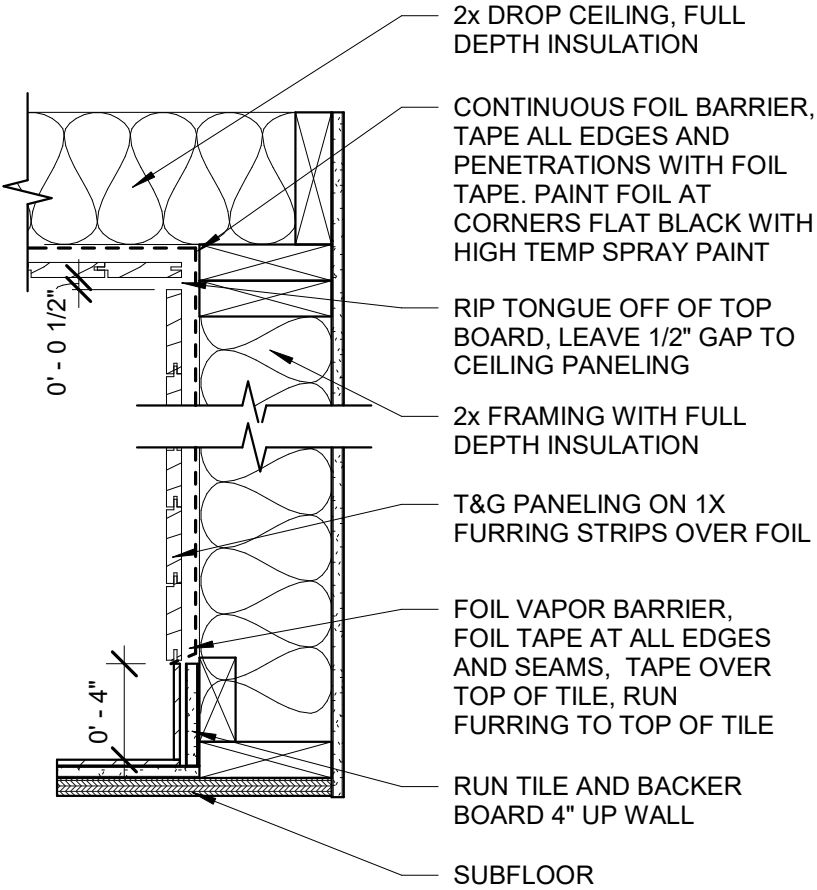
1 TYPICAL WALL DETAIL SKETCH 1 1/2" = 1'-0"
