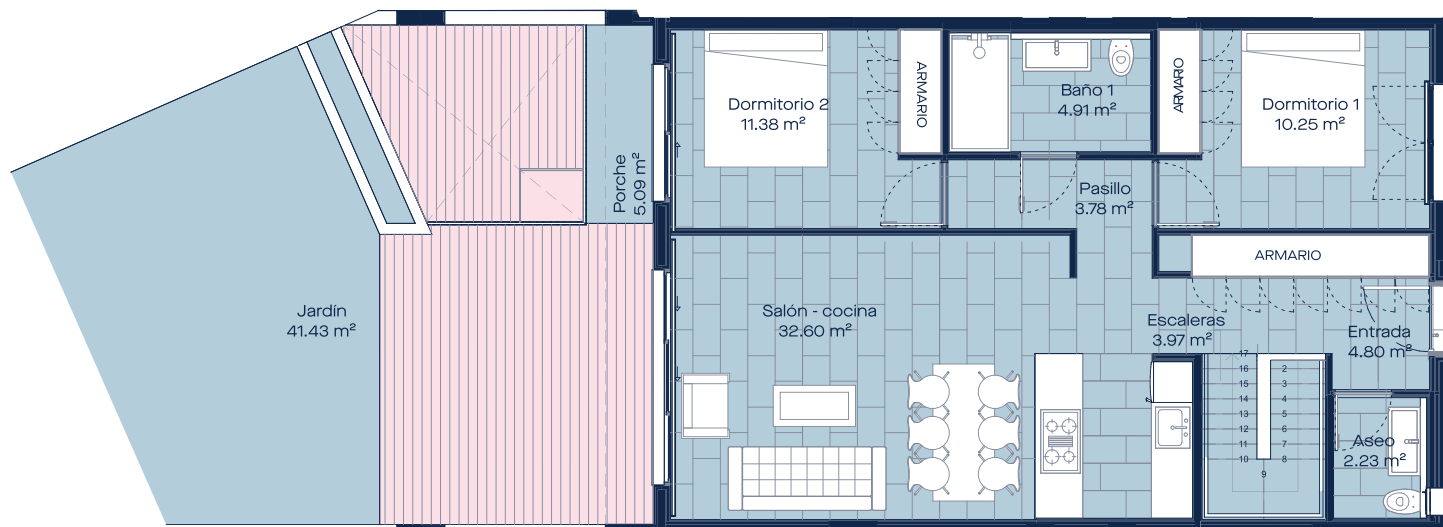
Planta Baja / GROUND FLOOR
