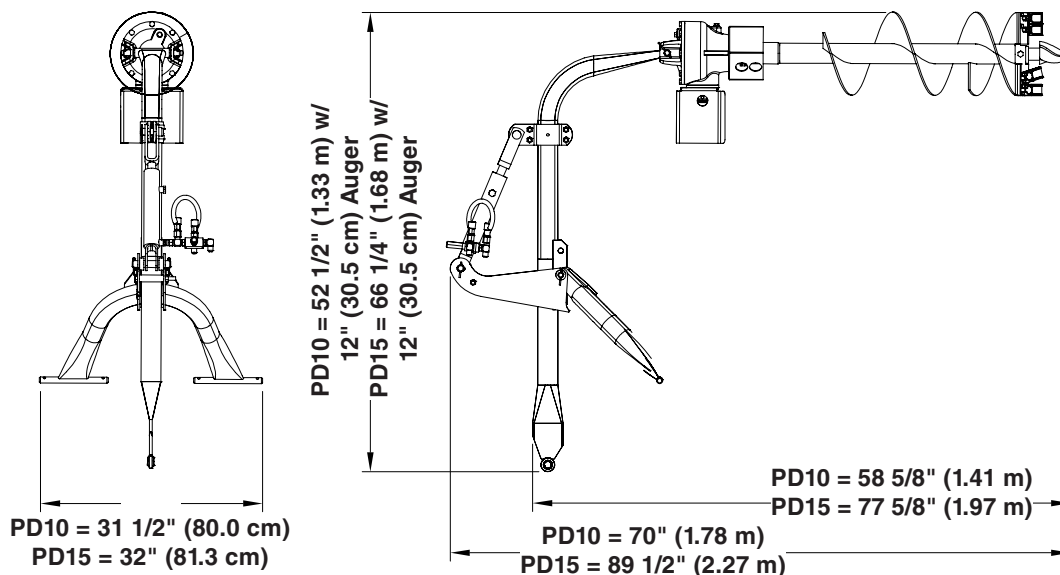
PD10 &amp; PD15 Overall Dimensional Drawing
