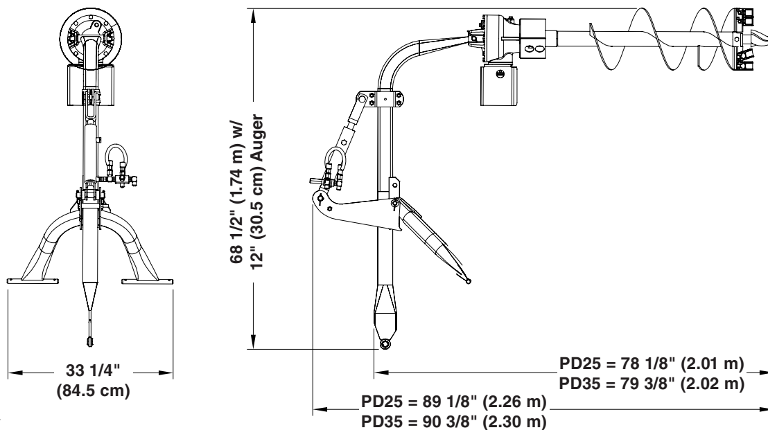
PD25 & PD35 Overall Dimensional Drawing
