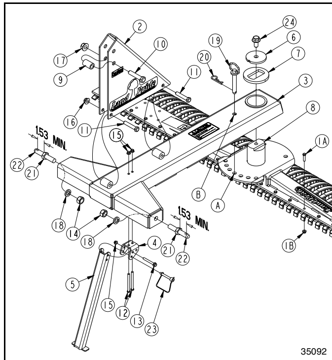
LR26 Series Landscape Rake Assembly Figure 1-2
