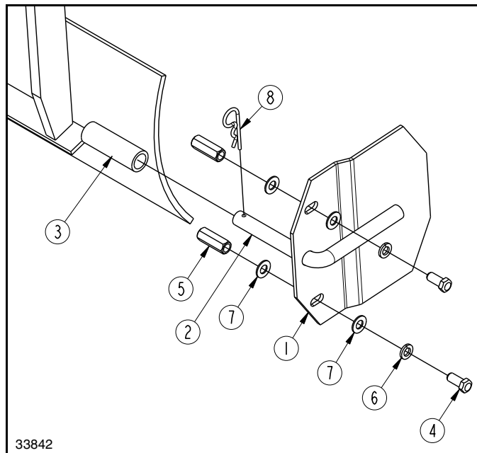
Side Plate Assembly Right-Hand Side shown Figure 2-5
