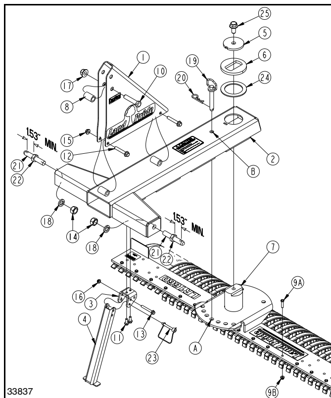
LR16 Series Landscape Rake Assembly
