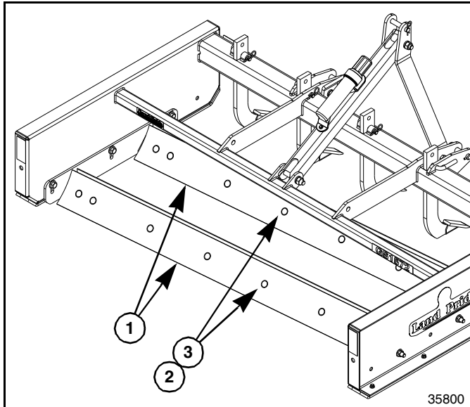
Rear Mounting Cutting Blades Figure 4-1
