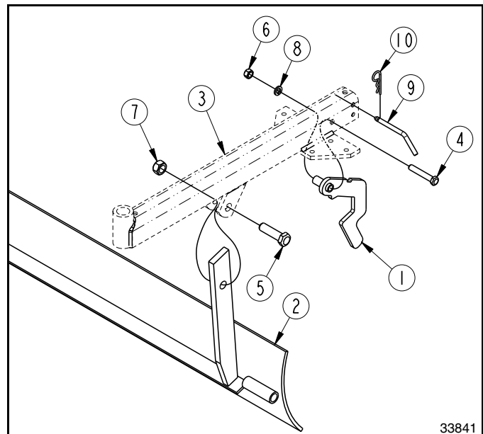
Grader Blade Assembly with Gauge Wheel Right-Hand Side Shown Figure 2-2
