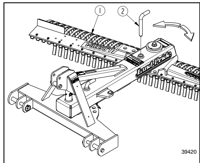
Rake Angling (manual shown) Figure 4-2
