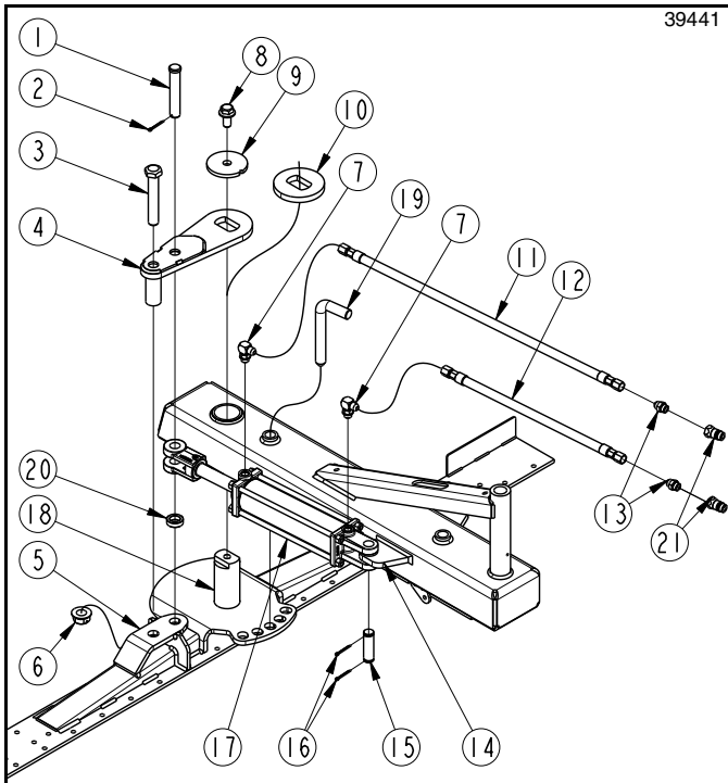
Hydraulic Angling Kit Figure 2-5
