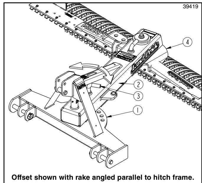
Rake Offset Figure 4-1
