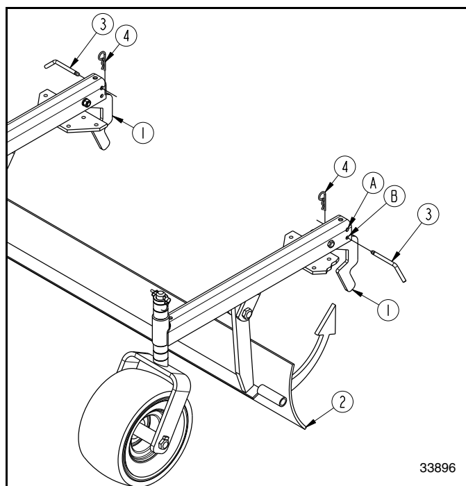
Grader Blade Lock Up Position Figure 4-4
