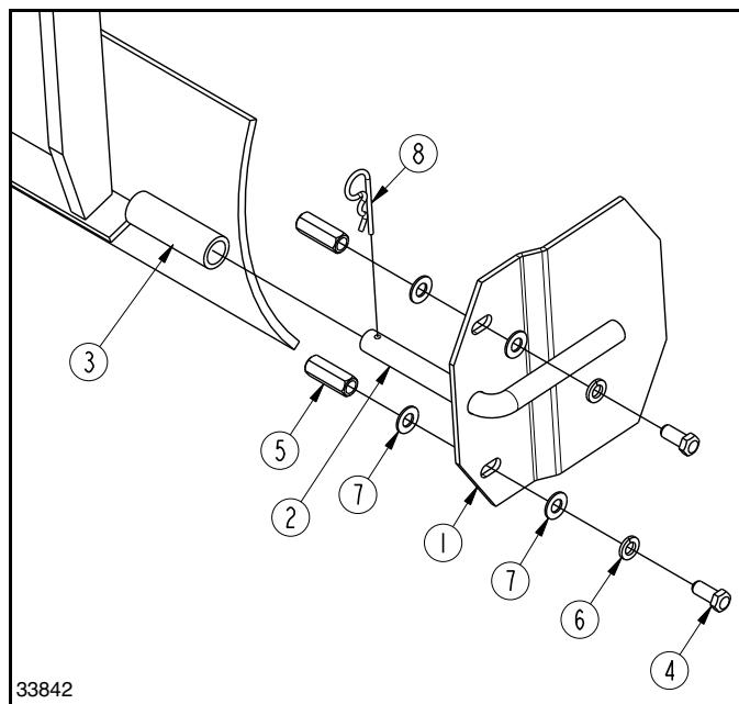
Side Plate Assembly Right-Hand Side shown Figure 2-4
