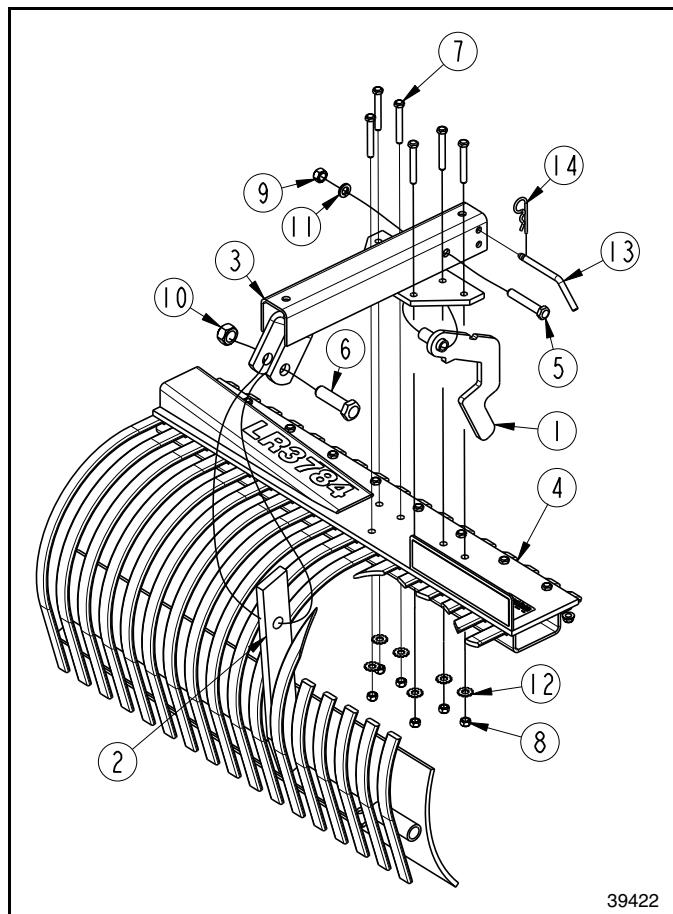
Grader Blade Assembly without Gauge Wheel Right-Hand Side Shown Figure 2-3
