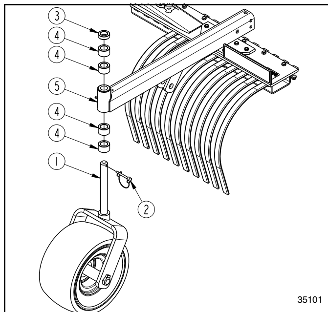
Gauge Wheel Adjustment Right-Hand Shown Figure 4-3
