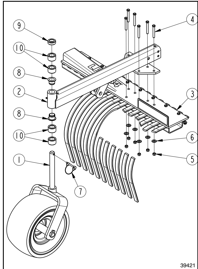
Dual Gauge Wheel Assembly Right-Hand Assembly Shown Figure 2-1
