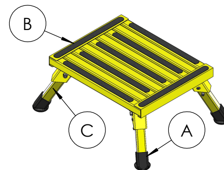
LEGS EXTENDED
