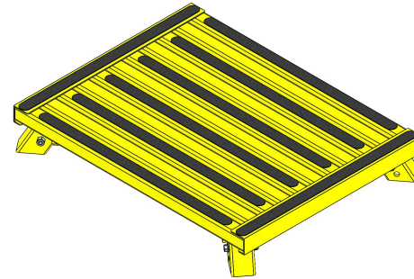
LEGS FOLDED
