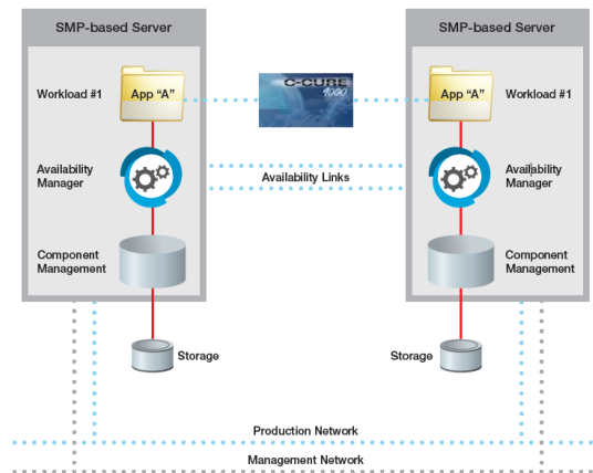
everRun Diagram
