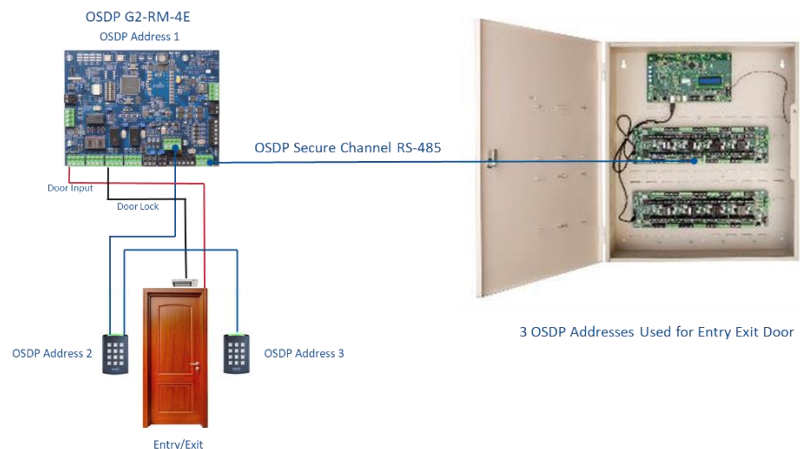
Typical high-level OSDP layout for an Entry/Exit door
