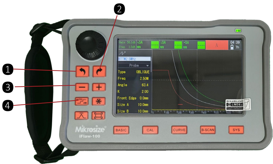
1.Back Key 2.Confirm Key 3.Decrease Key 4.Automatic Peak Adjustment Key
