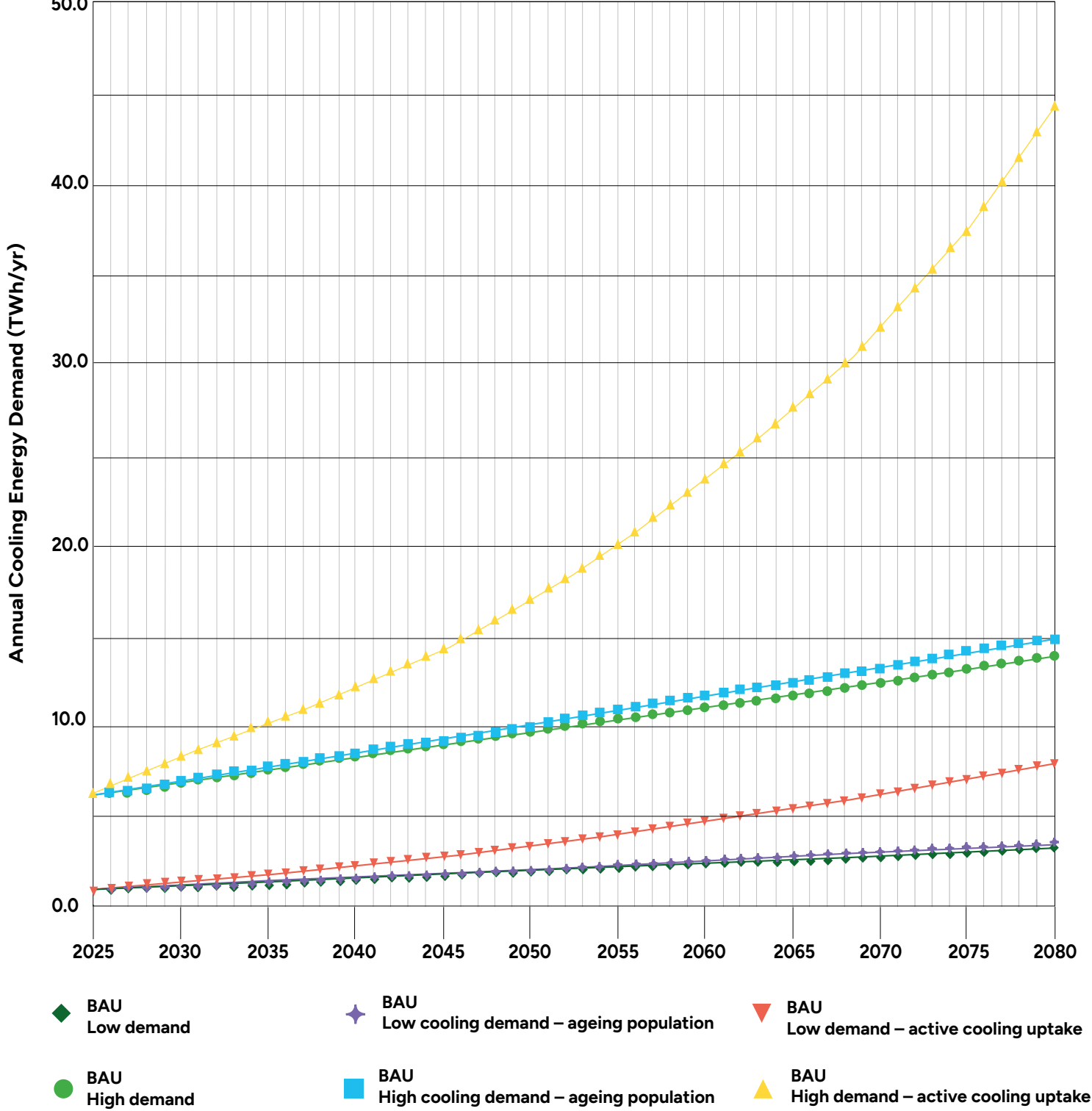
Figure 4: Baseline cooling energy demand projections for London from the BAR (2025-2080)
