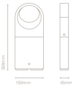
24430- with accessory 24491-Y
