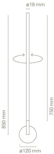
31177- Line Wall Vertical 850 mm
