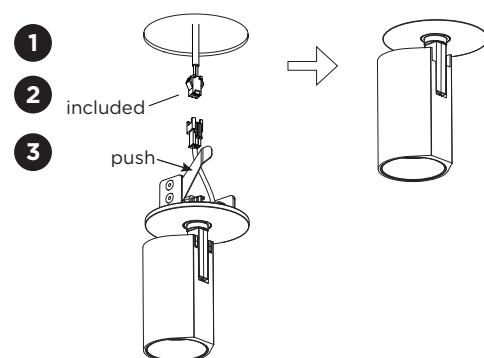
installation for 1.0 LED with blade springs
