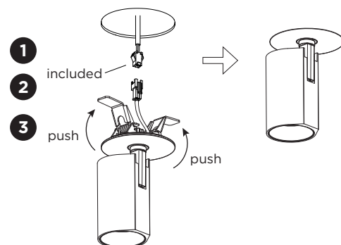
installation for 1.0 LED with wire springs
