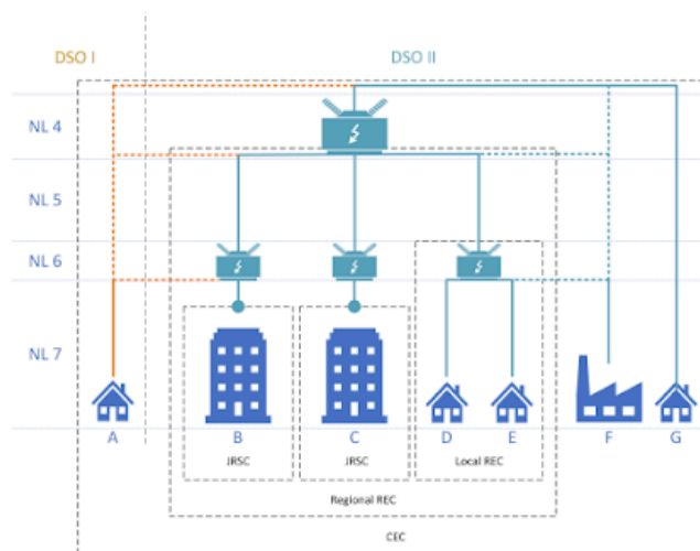
Figure 3: operational scopes for actors in the electricity systems in Austria 33
