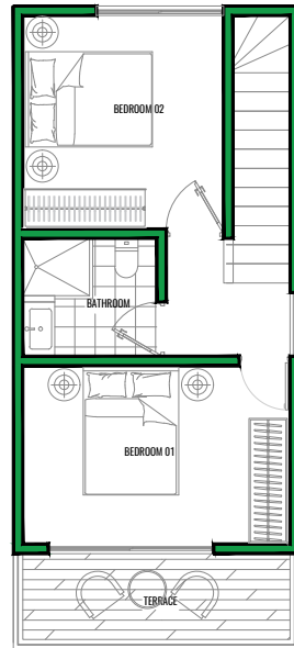
FLOOR PLAN (Second Floor)
