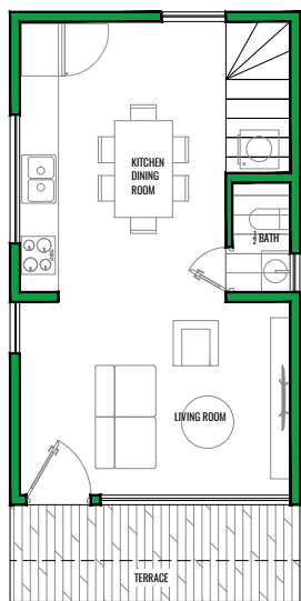
FLOOR PLAN (First Floor) Contemporary Two-Story Villa (1 BETHROOM)
