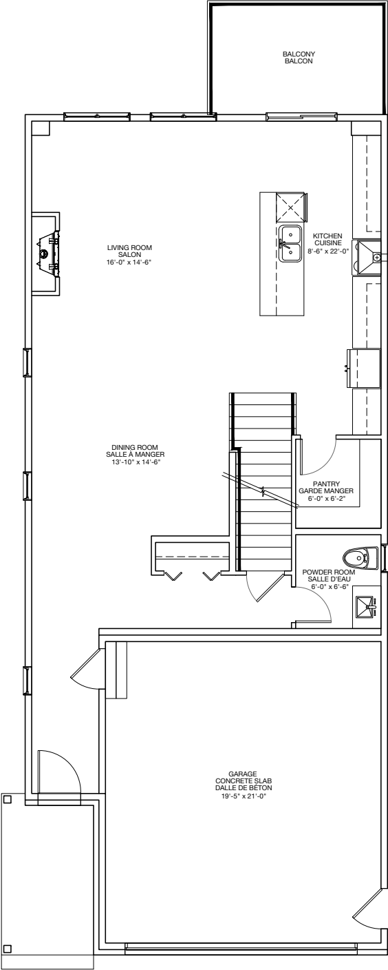
Ground floor Rez-de-chaussée
