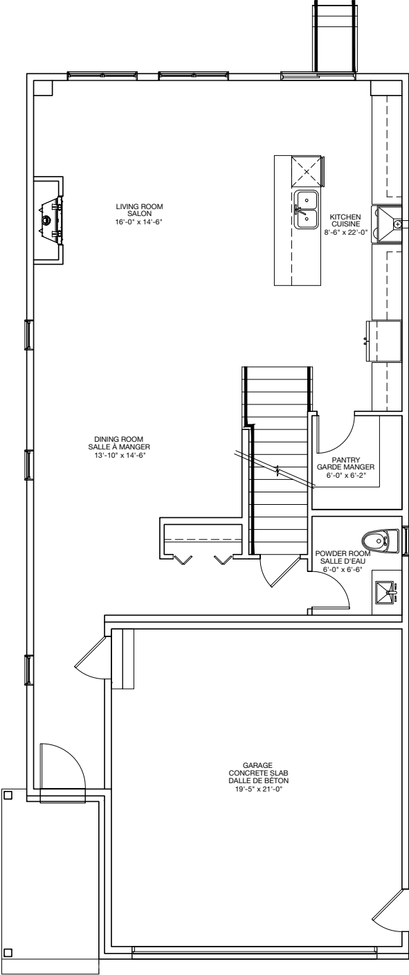
Ground floor Rez-de-chaussée
