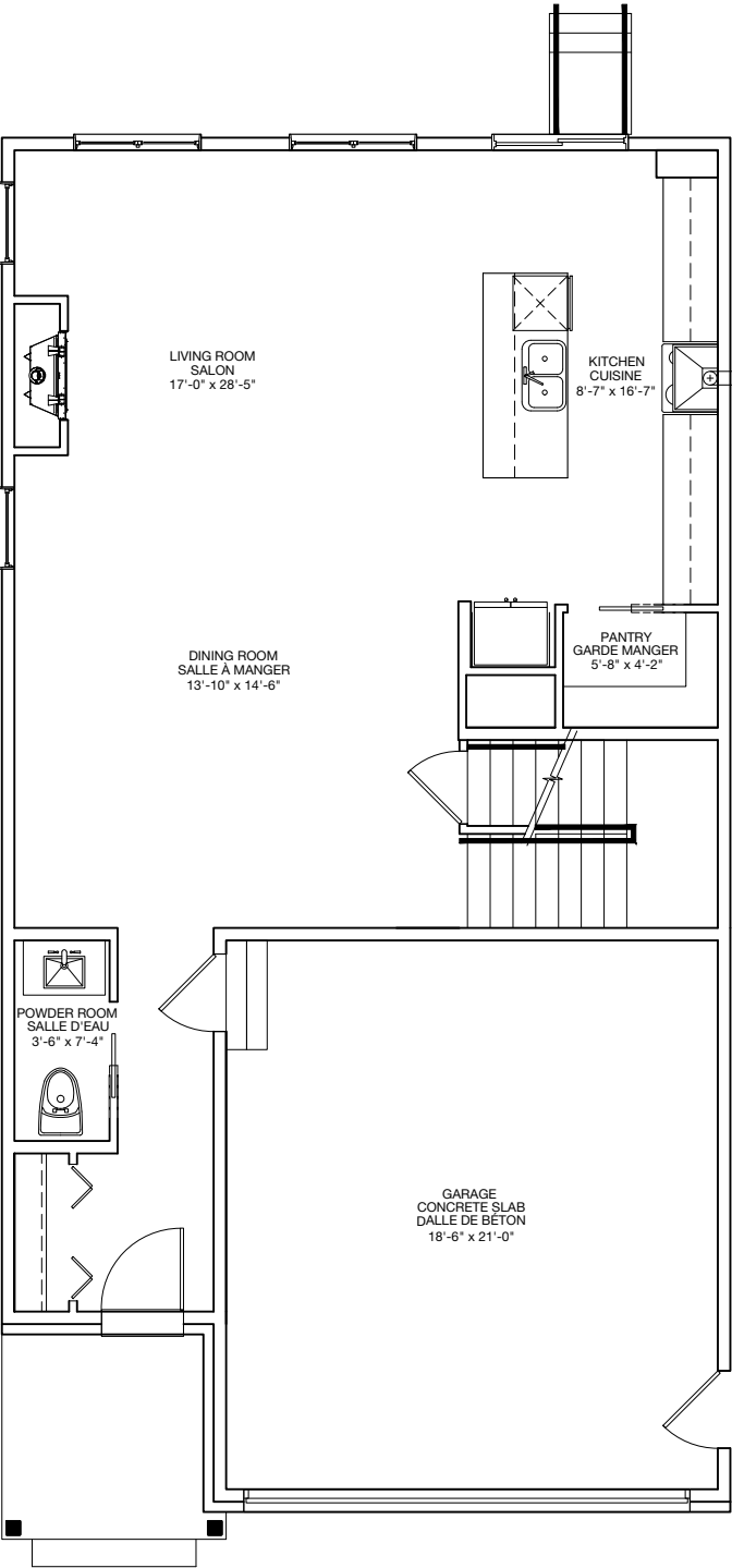
Ground floor Rez-de-chaussée
