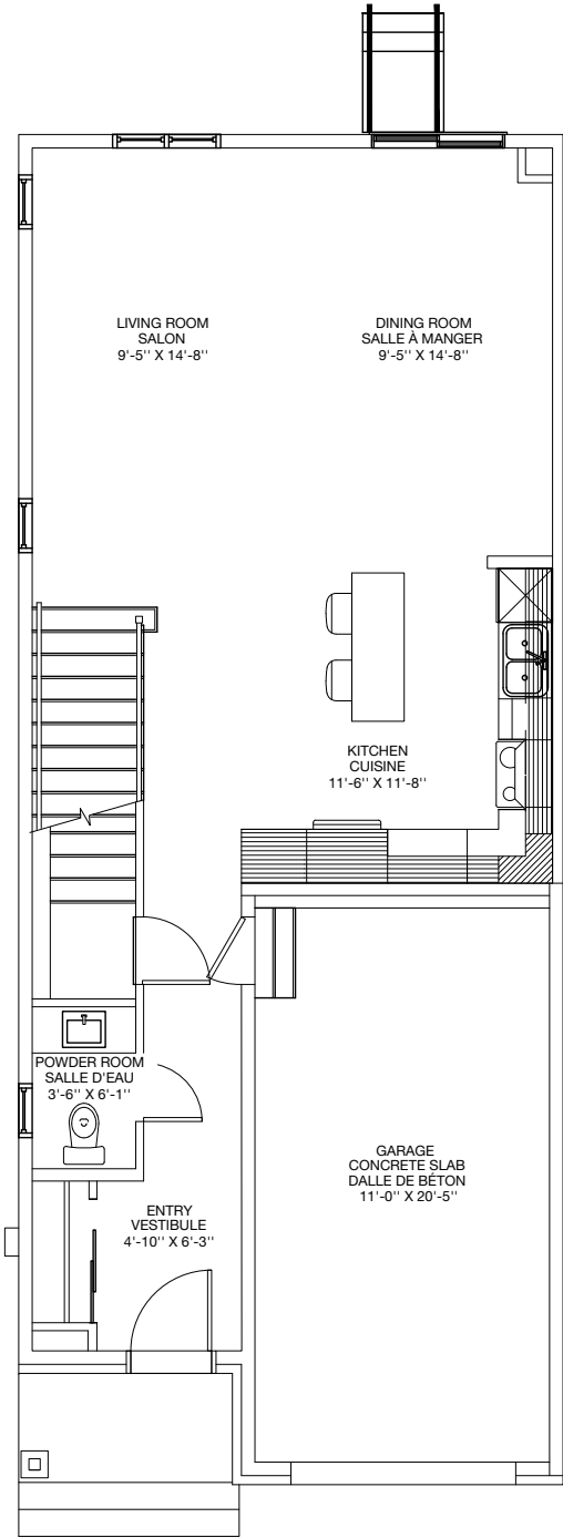
Ground floor Rez-de-chaussée
