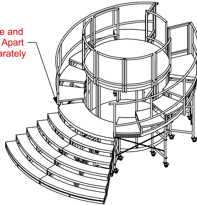
Iso View
