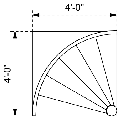
Top Plan
