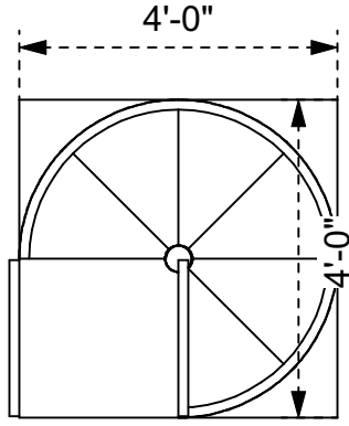
Top Plan
