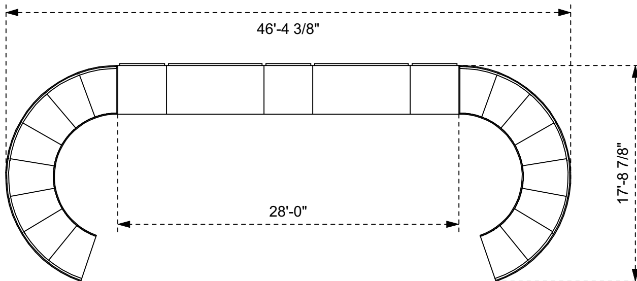
Top Plan
