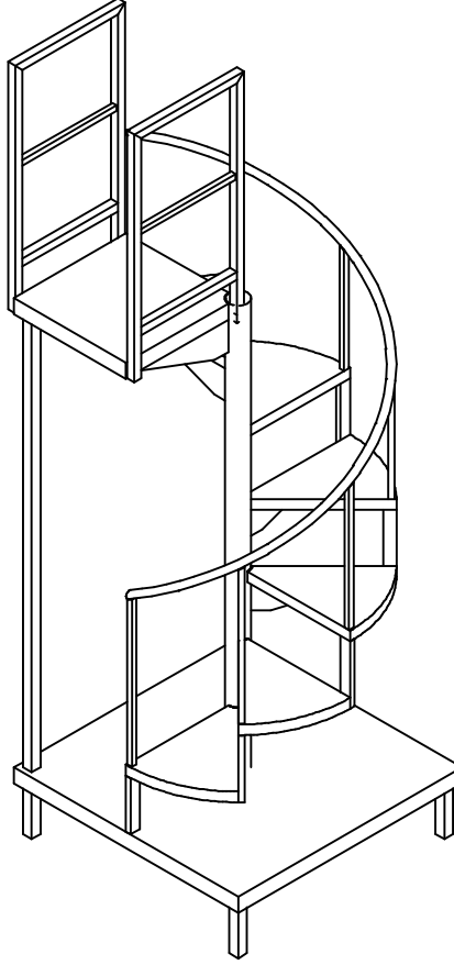
Iso View
