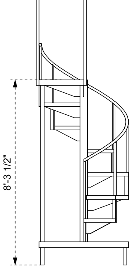
Front View
