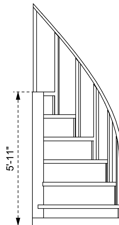
Right View
