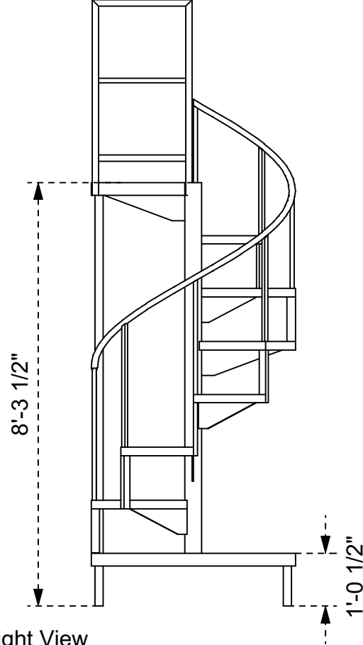
Right View
