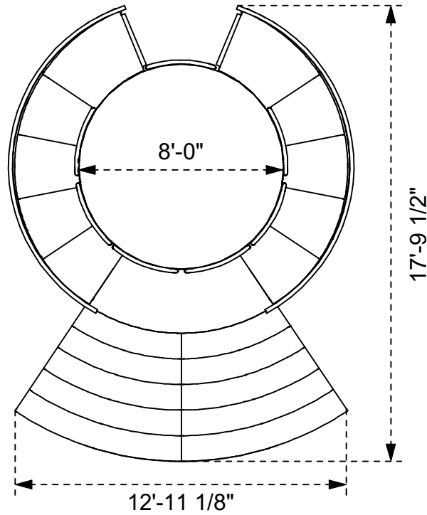
Top Plan
