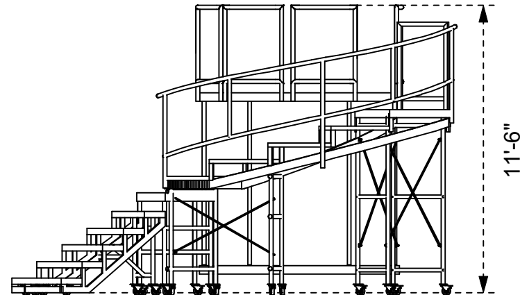
Right View
