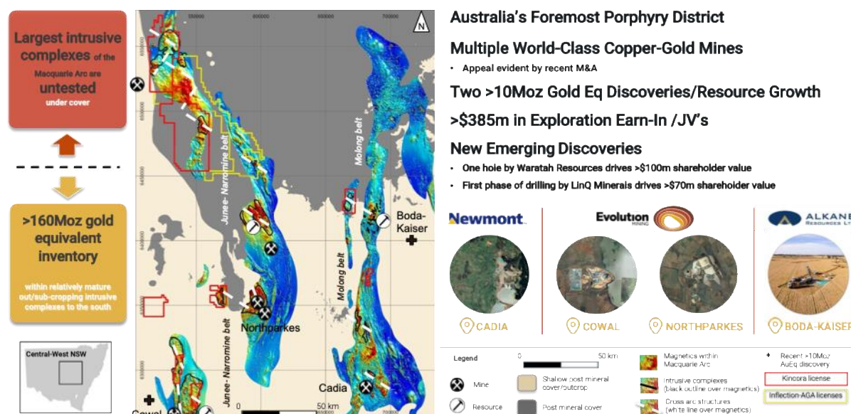
Figure 4: Magnetism maps Macquarie Arc volcanic belts, intrusive complexes and mineralised systems
