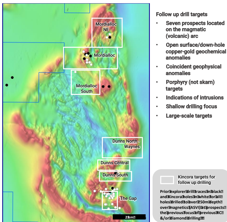
Figure 22: Seven large-scale, separate porphyry prospects currently identified by Kincora for follow up drilling
