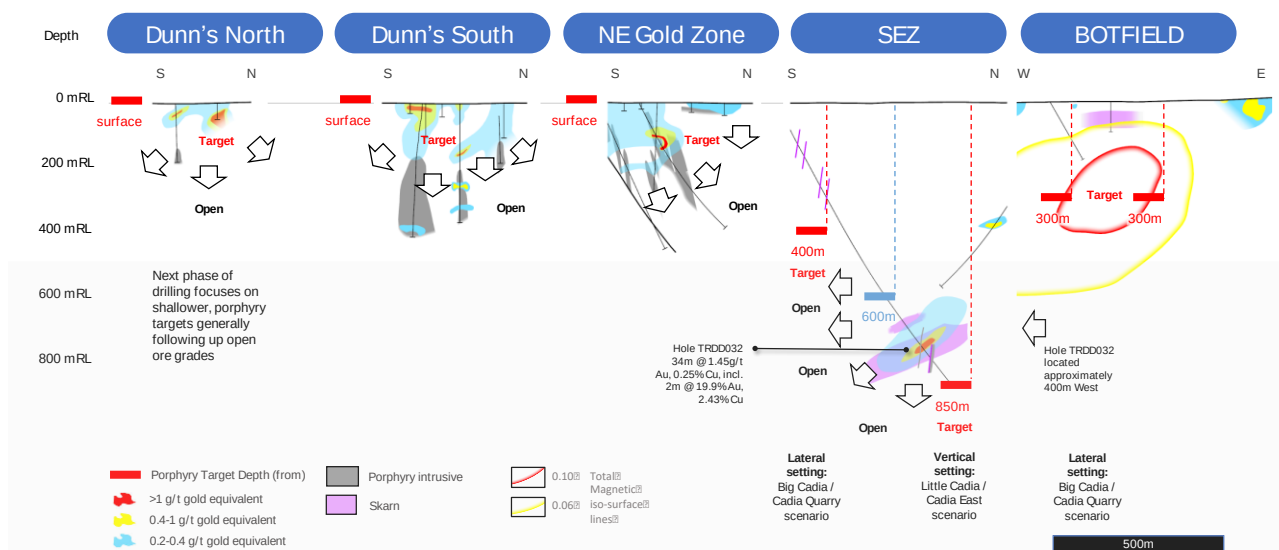
Figure 4: Next phase of drilling: illustration of target depths, open ore grade intervals and geological vectors
