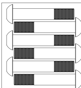
M10*55*20mm(25)-6pcs
