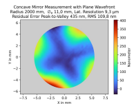
Residual error in comparison to the ideal mirror form: Slope values are measured, while height maps are generated via integration.
