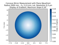
Large dynamic range of the instrument: The measurement of a concave mirror (Radius 2000 mm, 158 nm PV over 1") was performed with a plane wavefront.
