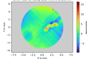
First Test for Repeatability - Error between two Measurements Flat Mirror, \phi_s 11,0 mm, Lateral Resolution 9,3 \mu m Error Peak-to-Valley 25,9 nm, RMS 2,1 nm
