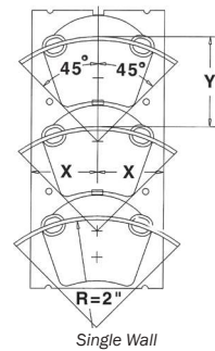
Single Wall
