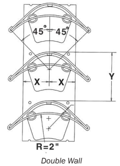
Double Wall
