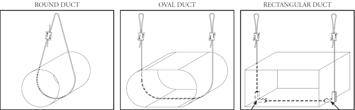
Rectangular Duct Corner Saddles Part No. HFCCS
