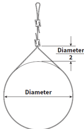
FIGURE 6—CABLE SHARK 125 (CS125) OR CABLE SHARK 250 (CS250) DEVICE LOCATION WHEN INSTALLED IN STANDARD LOOP CONFIGURATION
