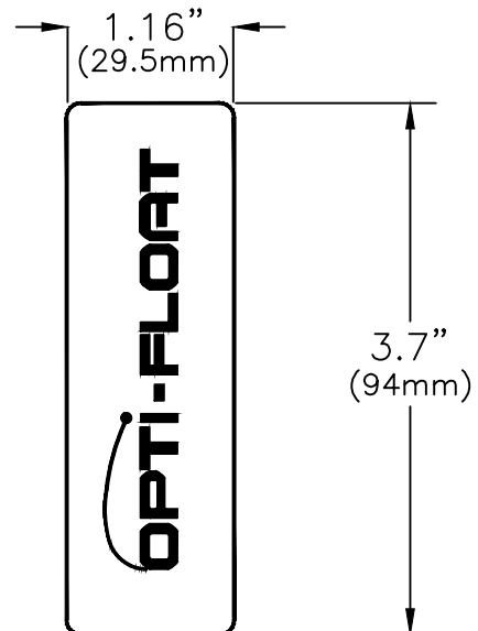
PAN VIEW
