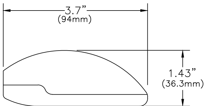
SIDE VIEW 2
