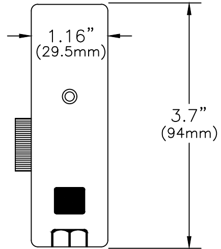
PAN VIEW
