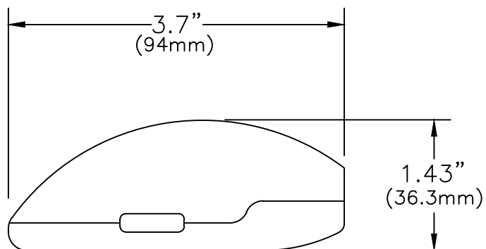
SIDE VIEW 1
