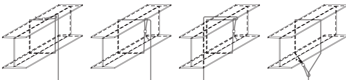
Prohibited Beam Hanging Configurations - See Approved Beam Hanging Configuration in Section 10 on Page 11.
