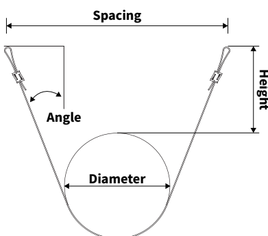
Spread Horseshoe Configuration Geometry
