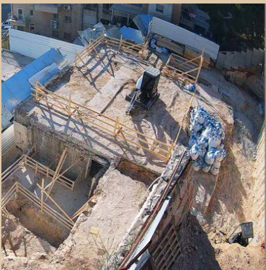
Foundations
