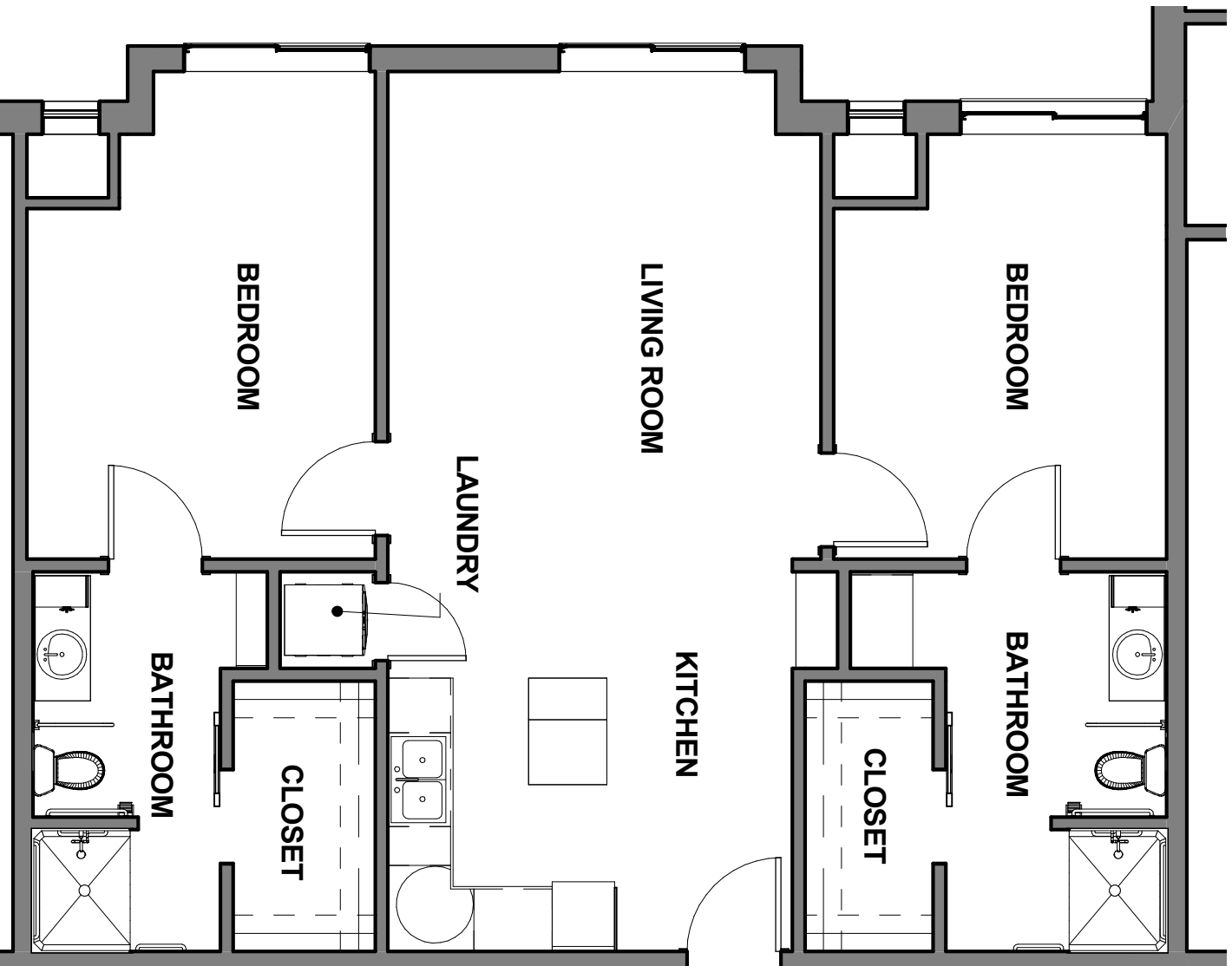
1 East AL Two Bedroom - 987 s.f. Z4 3/16" = 1'-0"
