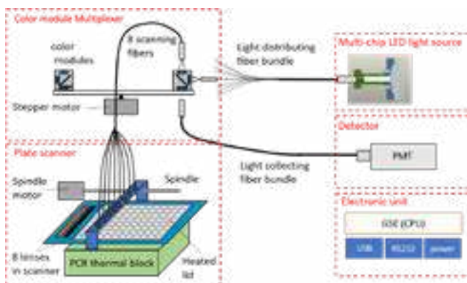
Patented fiber optic system - schematics for 96 well format
