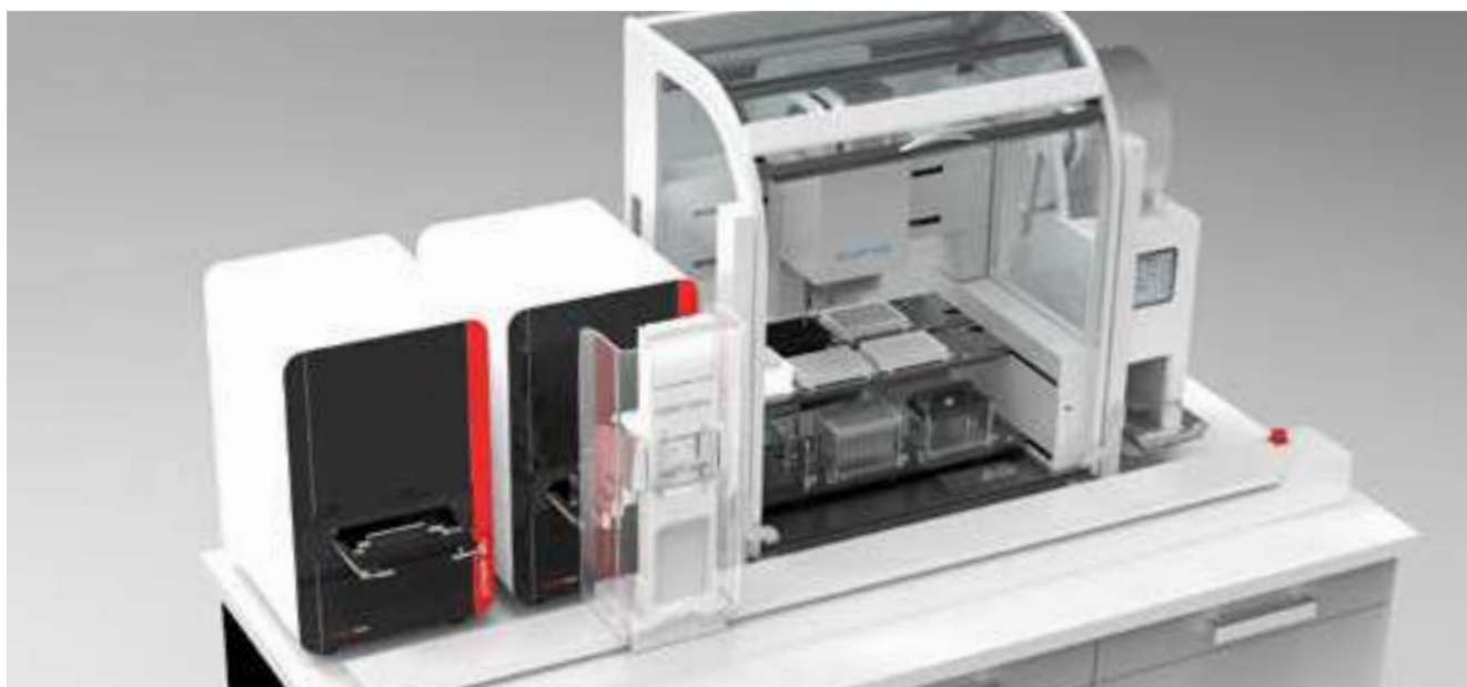
Representation of the fully automated qPCR workflow with 2 x qTOWER 3 auto real-time PCR cycler, including enhanced sample preparation (CyBio FeliX), transportation unit (CyBio Carry) and automated sealing (Agilent PlateLoc).
