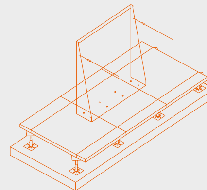
PLANTERLINE FIXED TO RAAFT® SUPPORT SYSTEM
