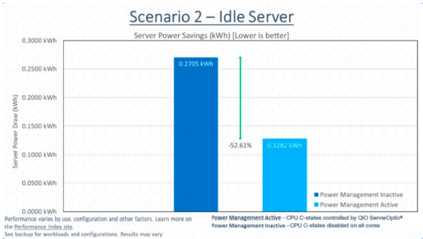
Figure 5. Idle Server Results
