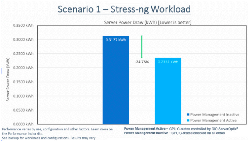
Figure 4. Stress-ng Workload Results
