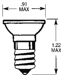
T-2 CANDELABRA SCREW BASE
