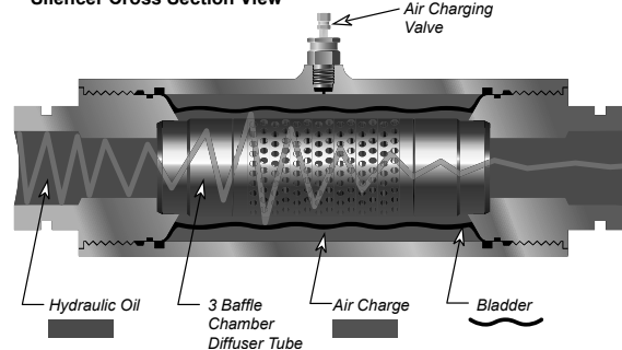
Silencer Cross Section View
