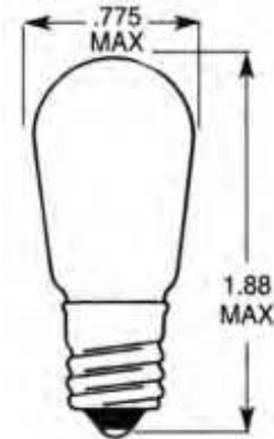
S-6 CANDELABRA SCREW BASE
