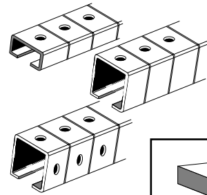
CHANNEL
