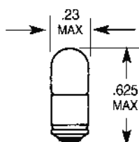
T-1.75 MIDGET GROOVED BASE
