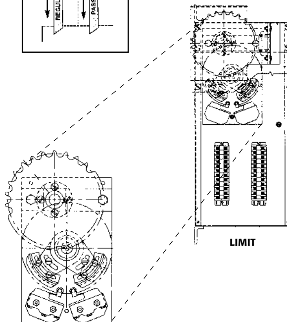
CAM CARRIER ASSEMBLY
