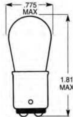
S-6 DOUBLE CONTACT BAYONET BASE
