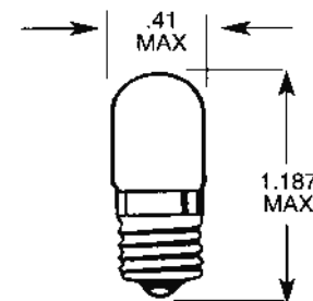
T-3.25 MINIATURE SCREW BASE
