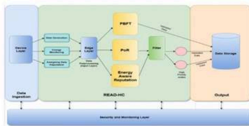
Fig. 2. Model Architecture
