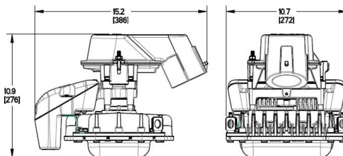
25° Standion Mount
