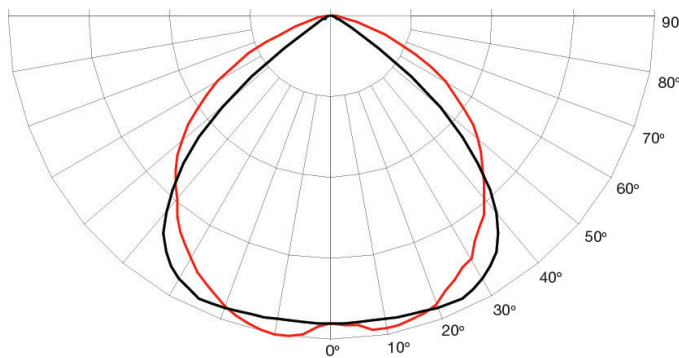
360° Beam Angle
