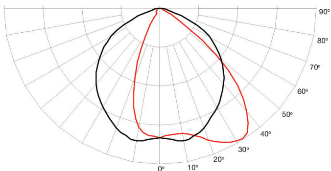
180° Beam Angle
