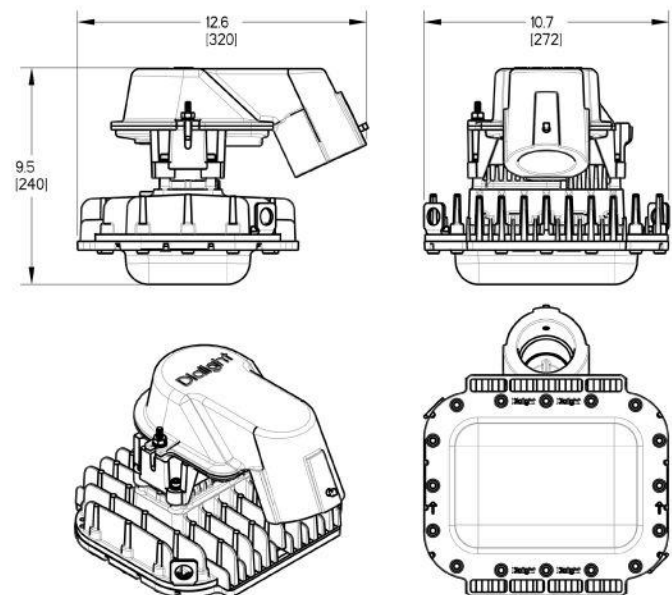
25° Stanchion Mount
