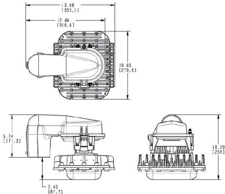
90° Stanchion Mount
