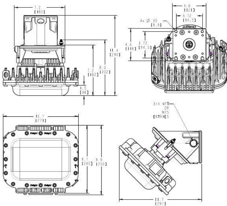
45° Wall Mount
