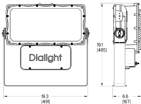
Prosire Floodlight Heavy Duty Bracket
