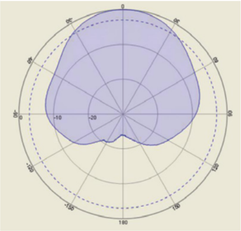
Radiation pattern
