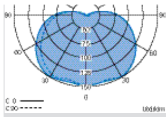
Polar curve 8W dKLK 23 LED
