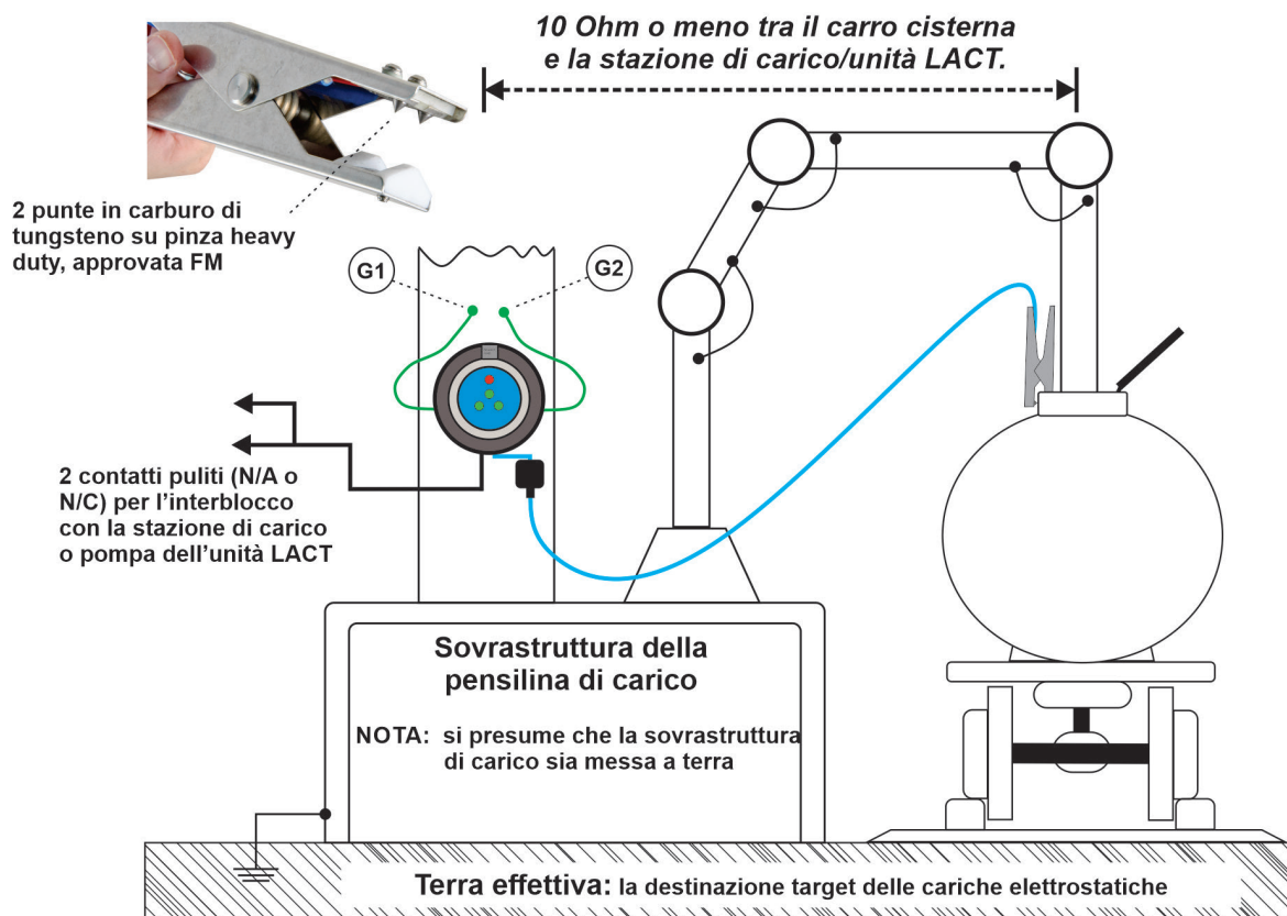
Fig. 2 - Typical Earth-Rite® PLUS rail tanker loading gantry installation. The tungsten carbide teeth on the grounding clamp are the contact points for the intrinsically safe signal that verifies if the rail tanker is grounded to the loading rack (or LACT unit) through connections G1 & G2 with a resistance of 10 Ohms or less
