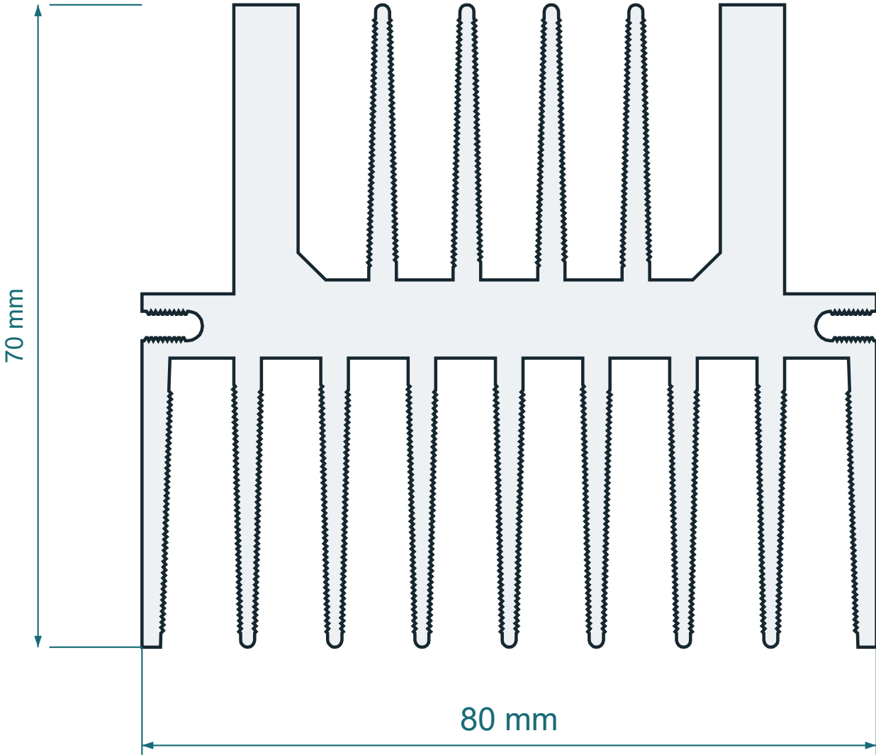
Central body: 7 mm. Double-sided fin structure.
