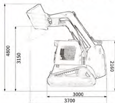
1.2Ton Skid Steer Loader OJ100-T
