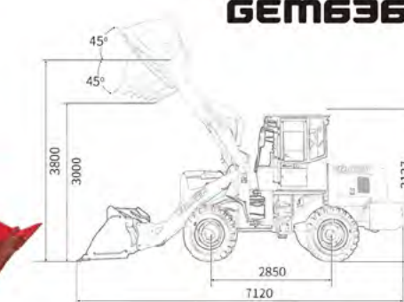
3.6Ton Wheel Loader GEM636
