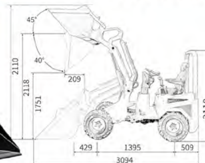
500kg Electric Loader WLE06
