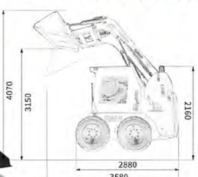
1.1Ton Skid Steer Loader OJ100-W
