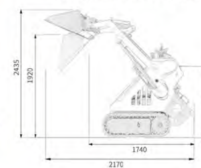
SK650 ELECTRIC 280kg Skid Steer Loader
