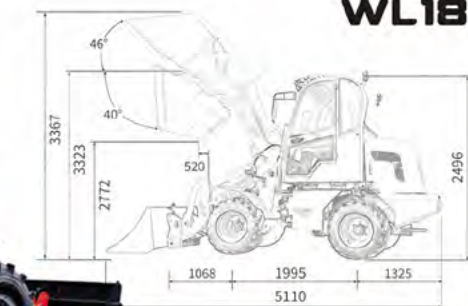
1.8Ton Wheel Loader WL18
