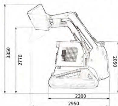
700kg Skid Steer Loader OJ50-T
