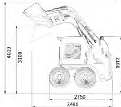
850kg Skid Steer Loader OJ60-W
